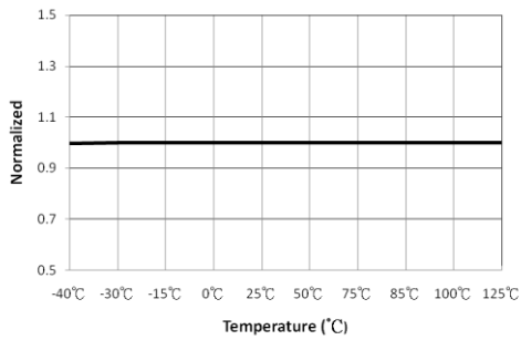
Figure 21. Reference Voltage for CV Regulation at 4.8 V ( V_{CVR-4.8V} ) vs. Temperature
