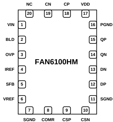
Figure 4. Pin Assignments
