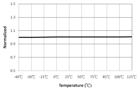
Figure 13. Voltage Difference between CSP and CSN at Mode 4 ( V_{CSP-CSN-M4} ) vs. Temperature
