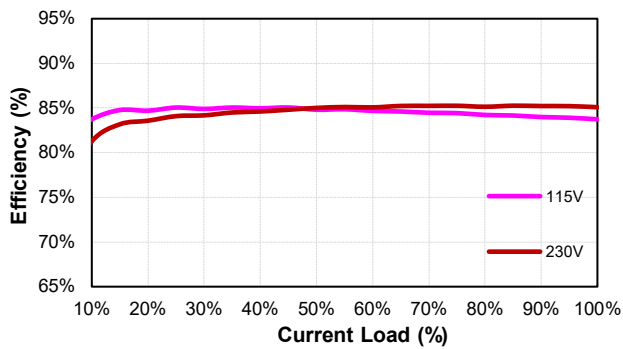
CFM40M090(Eff Vs Io)
