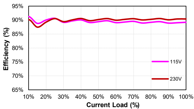
CFM40M480 (Eff Vs Io)
