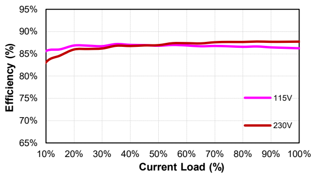
CFM40M150 (Eff Vs Io)
