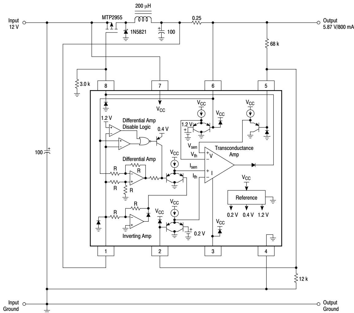
Figure 26 shows that the MC33341 can be configured as a high-side constant-current constant-voltage switch mode charger. This circuit operates as a step down converter. With a nominal input voltage and output load current as stated above, the switching frequency is approximately 28 kHz with an associated conversion efficiency of 86 percent. The switching frequency will vary with changes in input voltage and load current.
