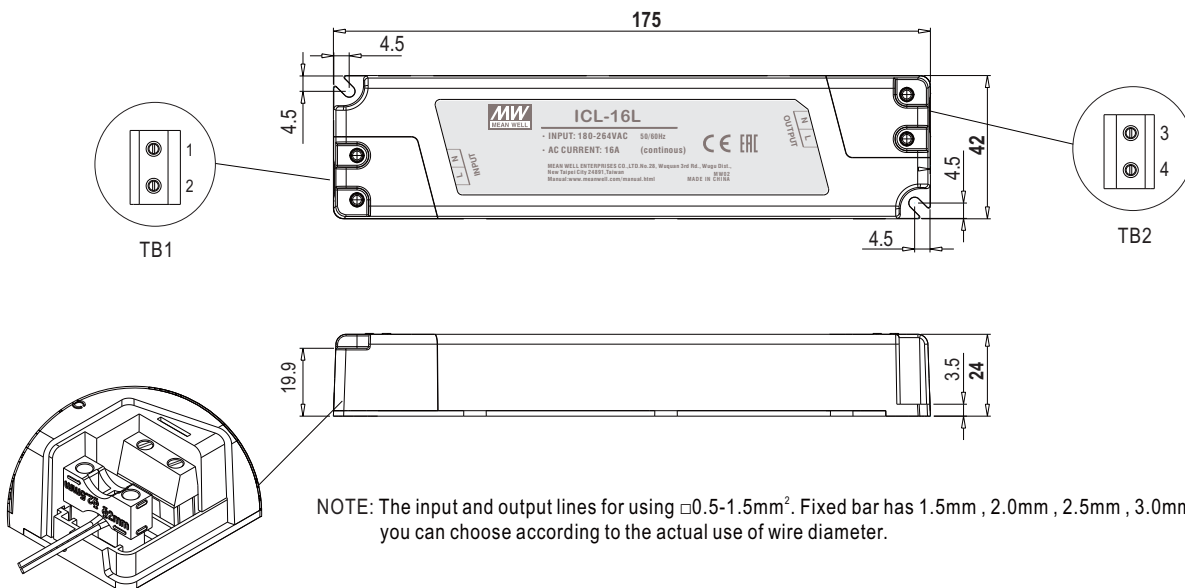
Terminal Pin No. Assignment (TB1,TB2)
