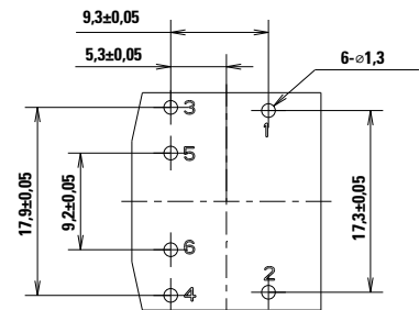
Piercing Plan
