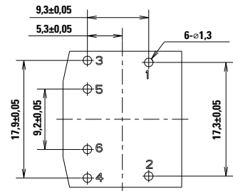
Piercing Plan
