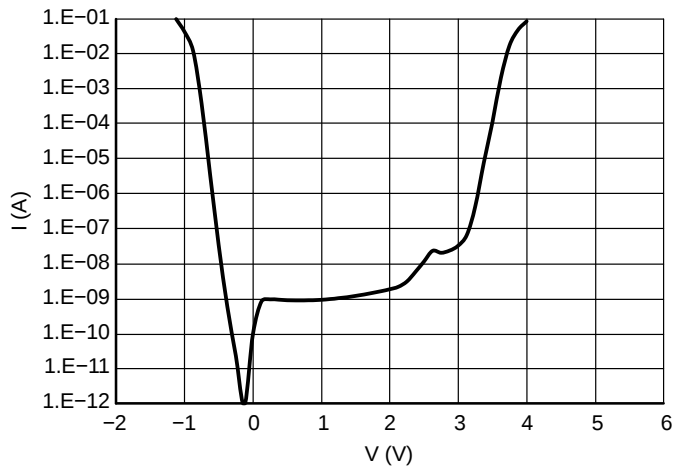
Figure 8. IV Characteristics
