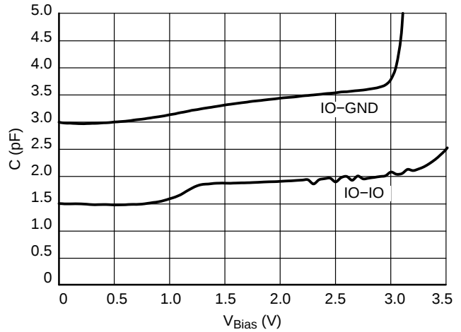
Figure 9. CV Characteristics
