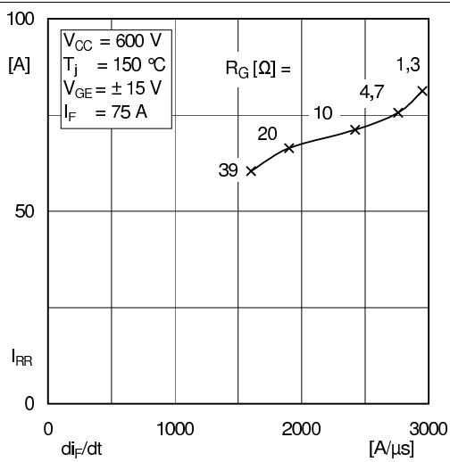
Fig. 11: CAL diode peak reverse recovery current
