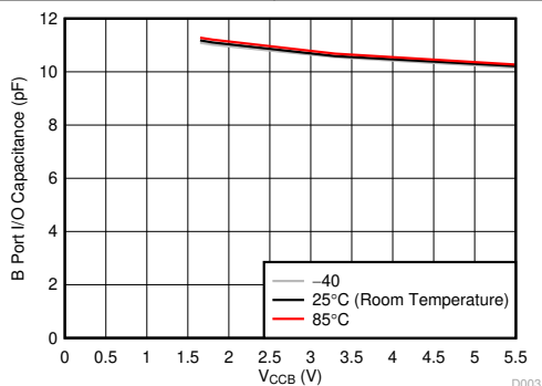
Figure 6-3. Capacitance for B Port I/O Pins ( C_{IO} ) vs Power Supply ( V_{CCB} )
