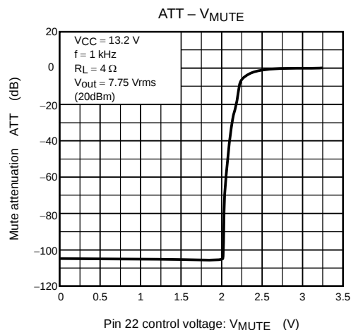
Figure 5 Mute Attenuation - V_{\text{MUTE}} (V)
