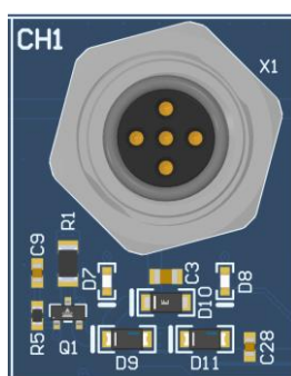
Figure 5. Channel 1
