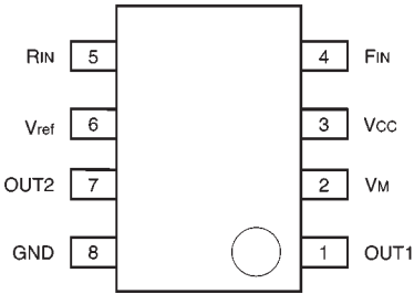
Fig.1 Pin assignments
