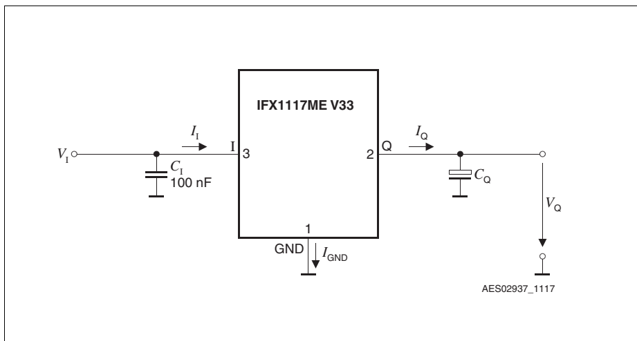
Figure 4 Measuring Circuit
