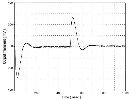
Fig.22 Output Load Transient Response 50% Load to/from 100% Load
