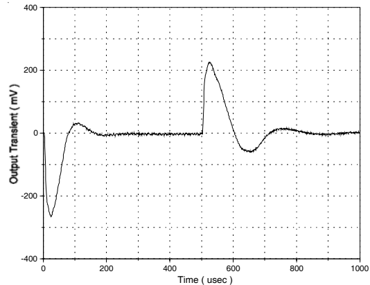
Fig.23 Output Load Transient Response 10% Load to/from 50% Load
