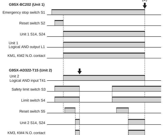
Timing chart 1
