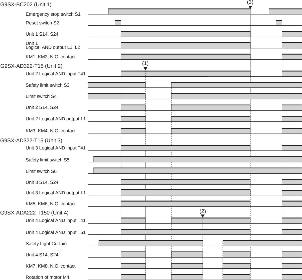
Timing chart 2
