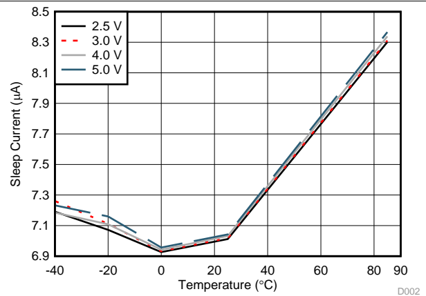
Figure 3. Sleep Current Across SDQ Voltage and Temperature
