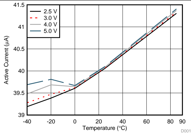
Figure 2. Active Current Across SDQ Voltage and Temperature (Not Authenticating)
