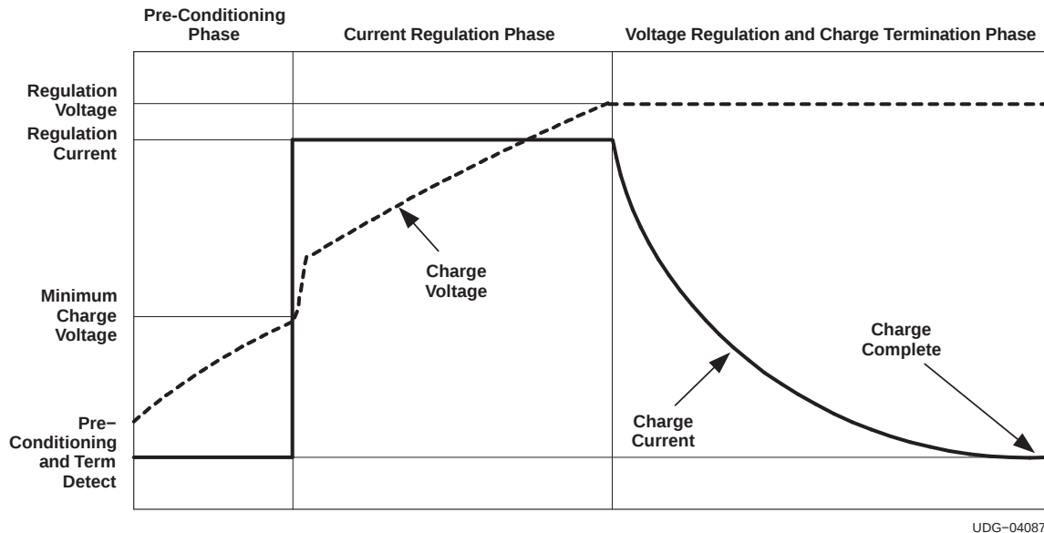
Figure 2. Charge Profile
