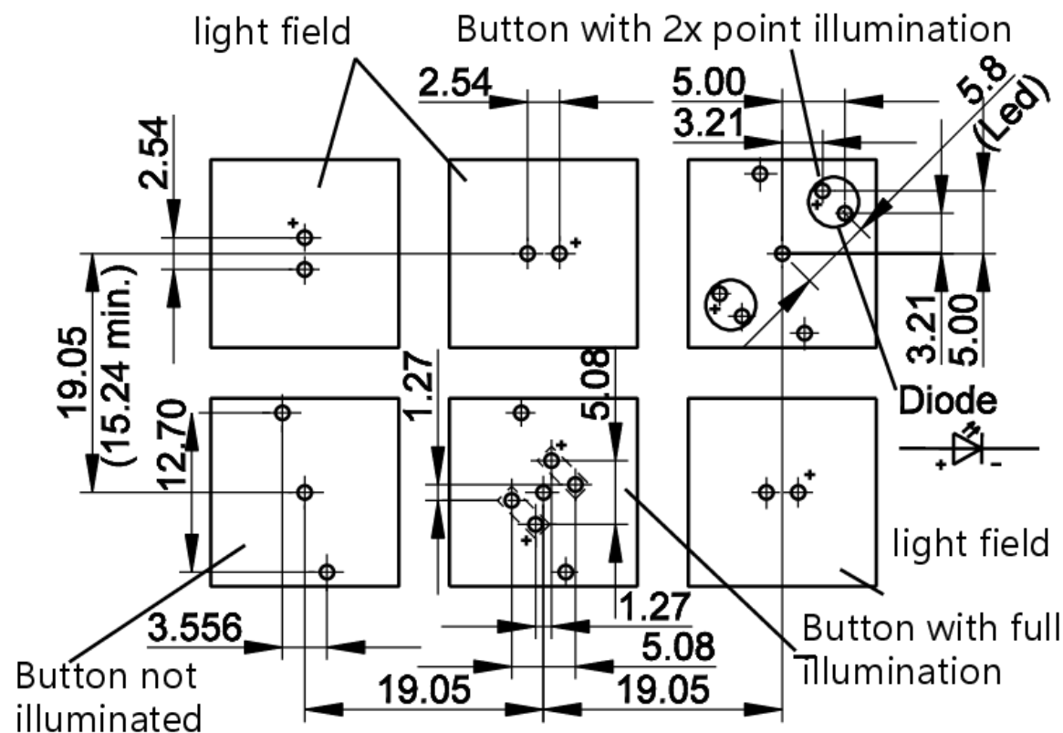
PCB drawing
