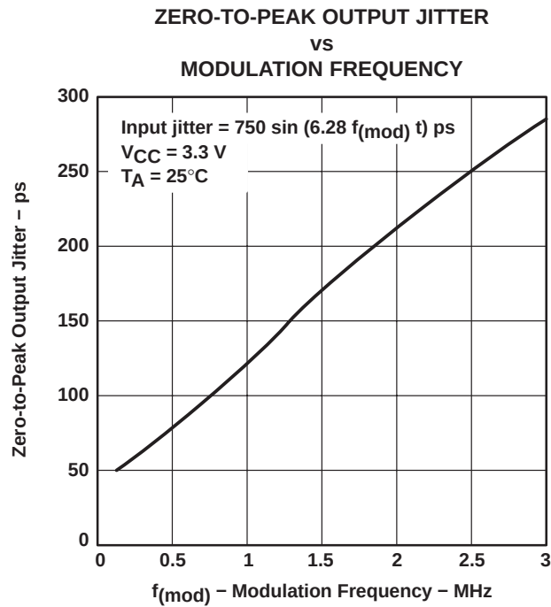
Figure 12. Typical FlatLink™ PLL Characteristics
