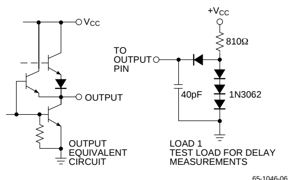
Figure 4. Output Circuits
