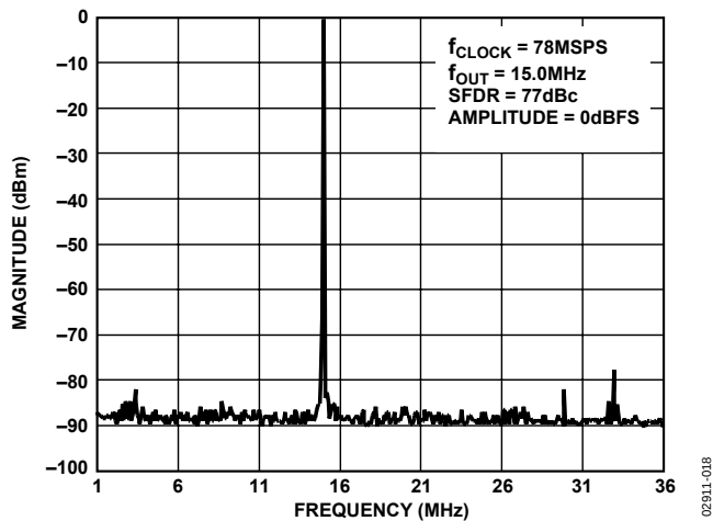
Figure 19. Single-Tone SFDR
