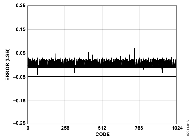
Figure 17. Typical DNL
