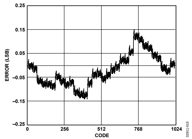
Figure 16. Typical INL
