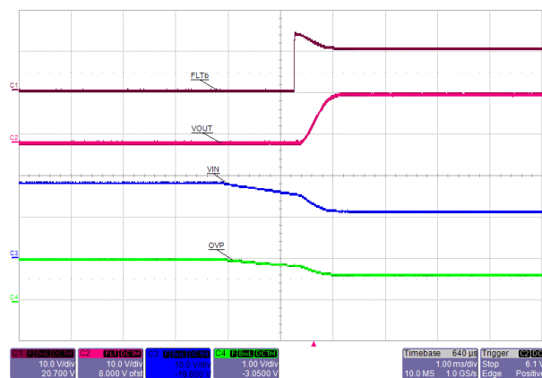
Figure 10-10. Overvoltage Recovery
