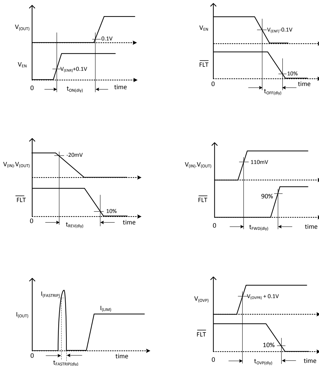
Figure 8-1. Timing Diagrams
