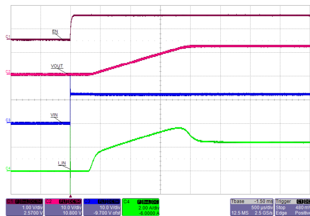
Figure 10-8. Hot-Plug Start-Up: Output Ramp With Start-Up Load of 4.8 Ω
