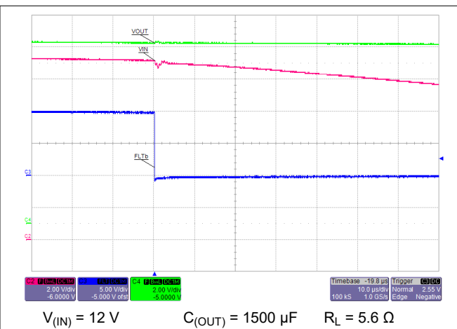
Figure 10-25. Hot-Plug Out Condition: FLT Delay
