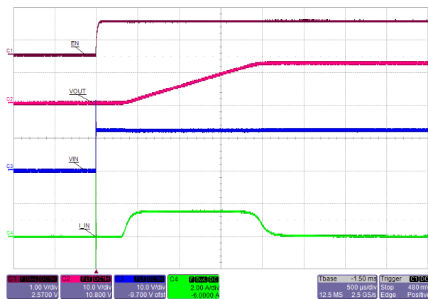
Figure 10-7. Hot-Plug Start-Up: Output Ramp Without Load on Output
