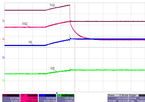
Figure 10-9. Overvoltage Shutdown
