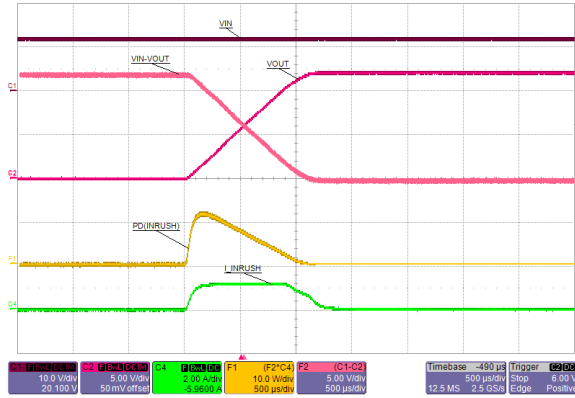
Figure 10-2. Start-Up Without Load
