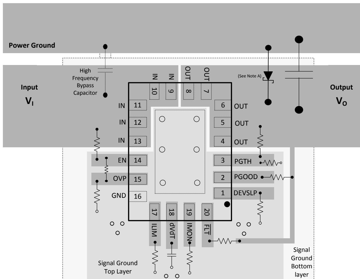
Figure 12-1. Board Layout
