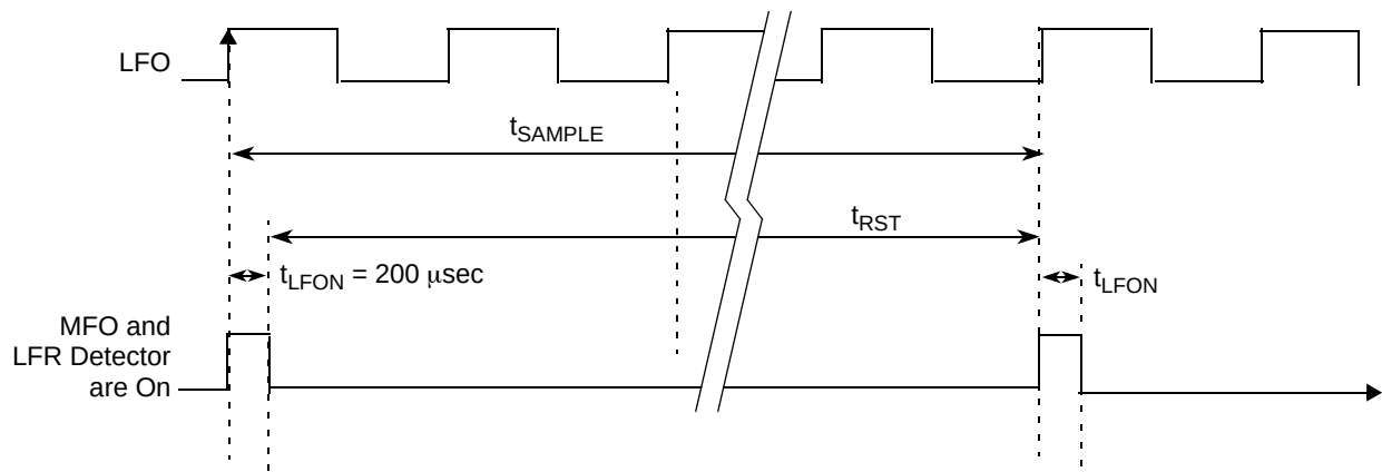
Figure 12-3 LFR Sample Timing - Carrier Detect Mode (LFON = 0 and no signal detected)
