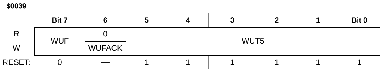
Figure 11-3 PWU Control/Status Register 0 (PWUCS0)
