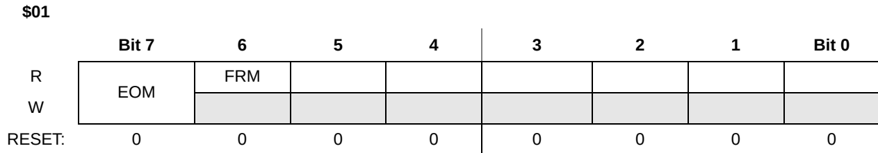
Figure 13-10 RFX Control Register 1 (RFCR1)
