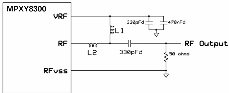
Output Power Measurement Configuration
