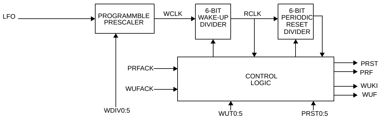
Figure 11-1 Wake-Up Timer Block Diagram
