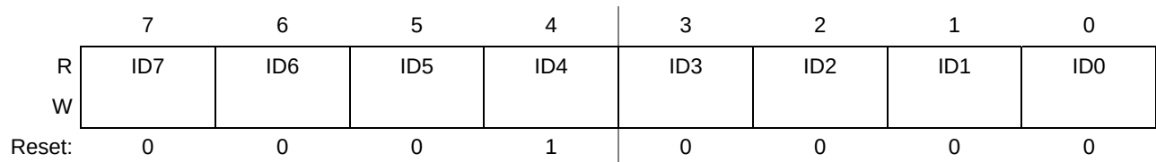
Figure 5-9 System Device Identification Register — Low (SDIDL)
