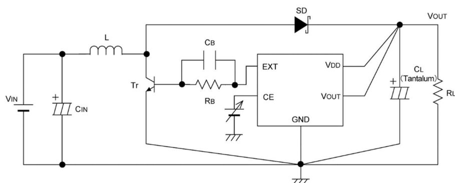
Circuit 7. XC6367A, XC6368A (NPN Transistor)
