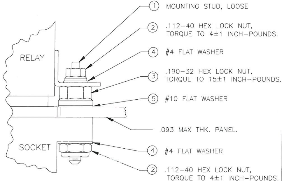
MOUNTING HARDWARE INSTALLATION SEQUENCE BY ITEM NUMBER TYP 3 PLACES
