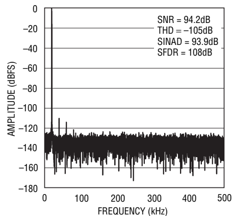
Figure 5. 16k Point FFT of the LTC2393-16, f_s = 1\text{Msps} , f_{IN} = 20\text{kHz}
