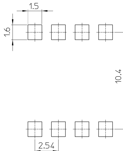
Fig. 14.2 Lead forming and taping option (LF4), (TP4)
