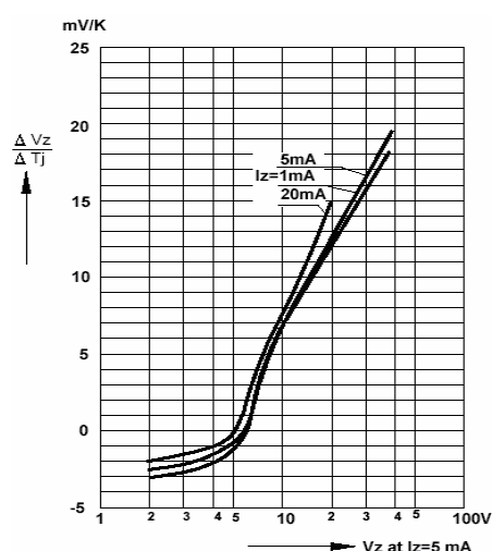
Fig 12. Temperature Dependence of Zener Voltage vs Zener Voltage
