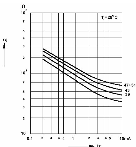
Fig 9. Dynamic Resistance vs Zener Current
