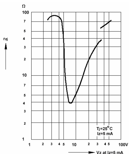
Fig 11. Dynamic Resistance vs Zener Voltage
