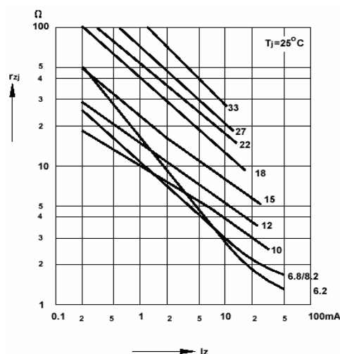
Fig 8. Dynamic Resistance vs Zener Current
