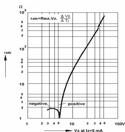
Fig 10. Thermal Differential Resistance vs Zener Voltage
