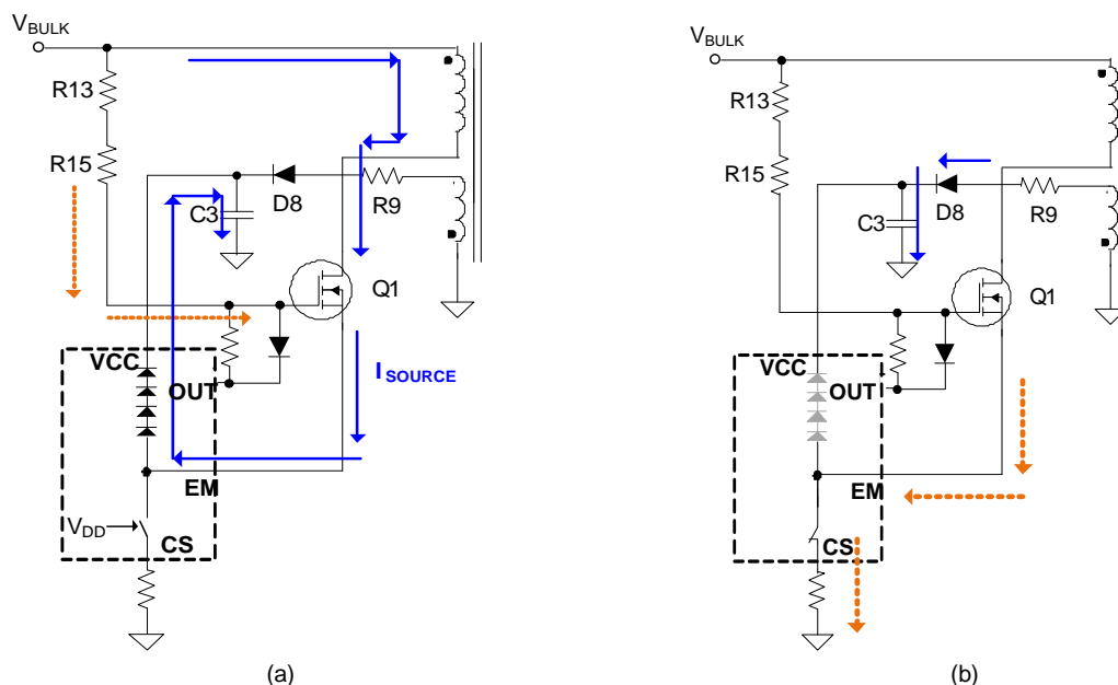
Figure 1. Start-up Circuit
