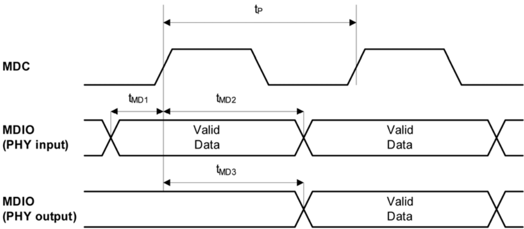
Figure 17. MDC/MDIO Timing
