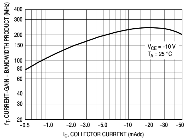
Figure 6. Current-Gain-Bandwidth Product
