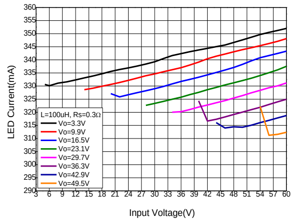
LED Current vs. Input Voltage ( R_S = 0.3\Omega , L = 100\mu\text{H} )
