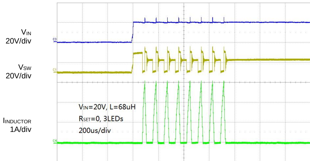
Figure 3. System Start up with Sense Resistor Short-circuit
