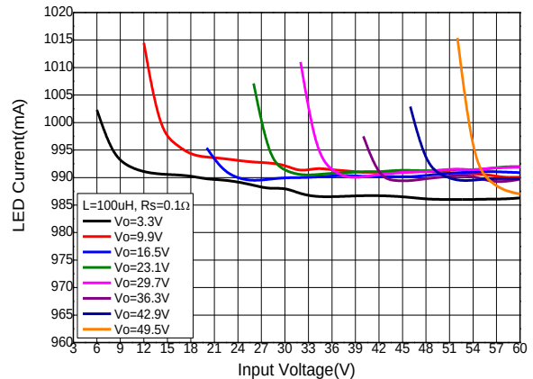
LED Current vs. Input Voltage ( R_S = 0.1\Omega , L = 100\mu\text{H} )
