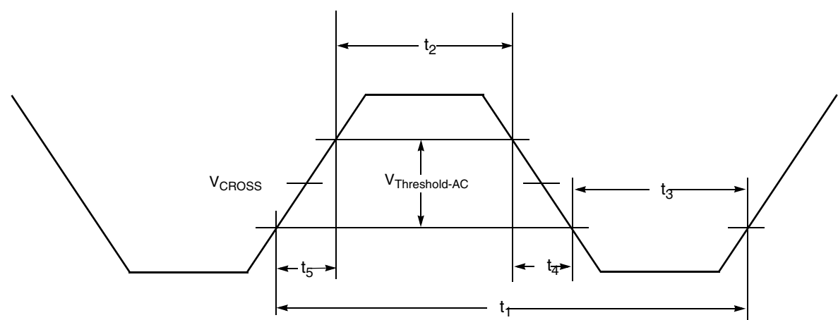
Figure 5-3. SYCLK Waveform
