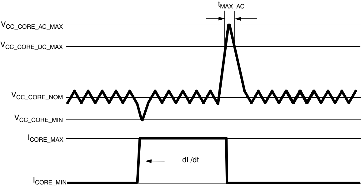
Figure 5-1. V CC_CORE Voltage Waveform
