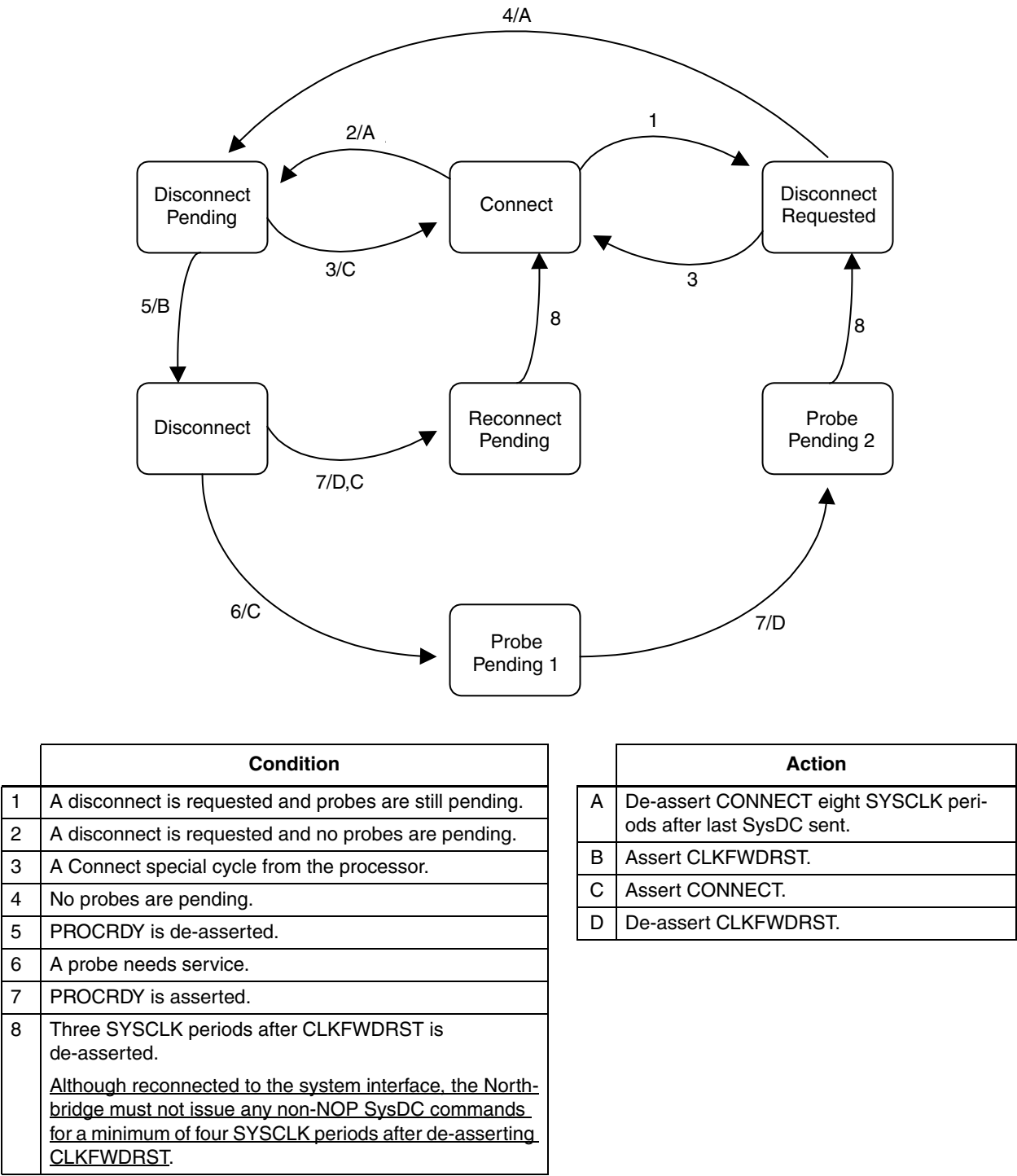
Figure 3-5. Northbridge Connect State Diagram
