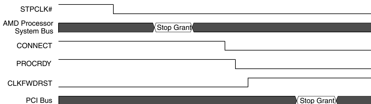
Figure 3-3. AMD Processor System Bus Disconnect Sequence in the Stop Grant State
