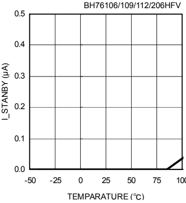
Fig.16 Temperature-Standby Circuit Current
