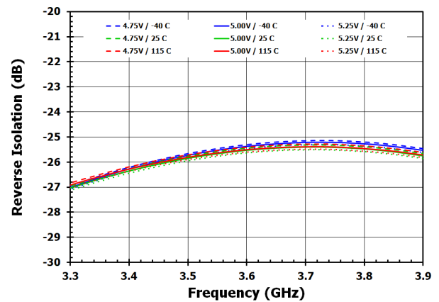
Figure 11. Reverse Isolation
