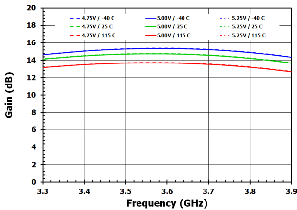
Figure 10. Gain
