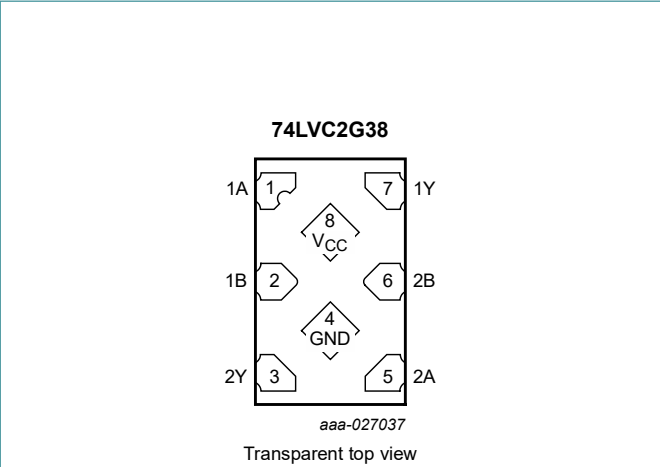
Fig. 7. Pin configuration SOT1233-2 (X2SON8)
