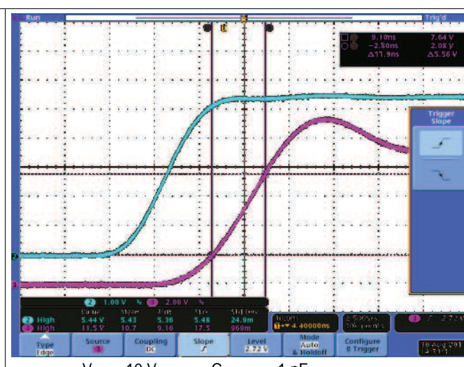
Figure 27. Typical Turnoff Waveform
