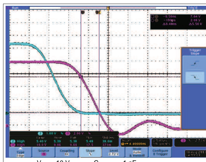
Figure 26. Typical Turnon Waveform
