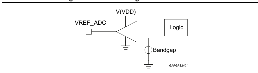
Figure 19. Internal voltage reference for ADC
