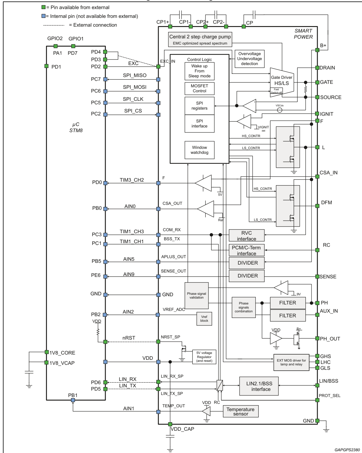
Figure 3. Block diagram
