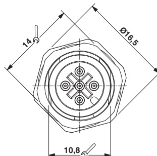
Dimensional drawing
