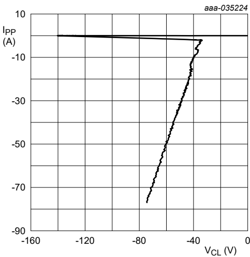
Fig. 7. Dynamic resistance with negative clamping; typical values
