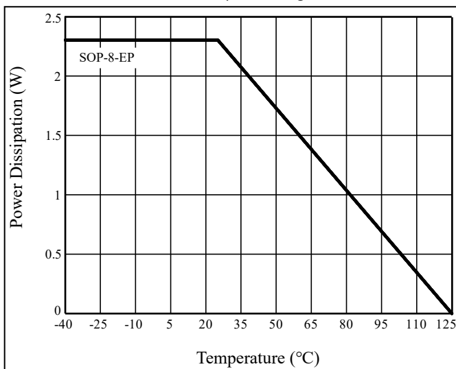
Figure 30 Dissipation Curve
