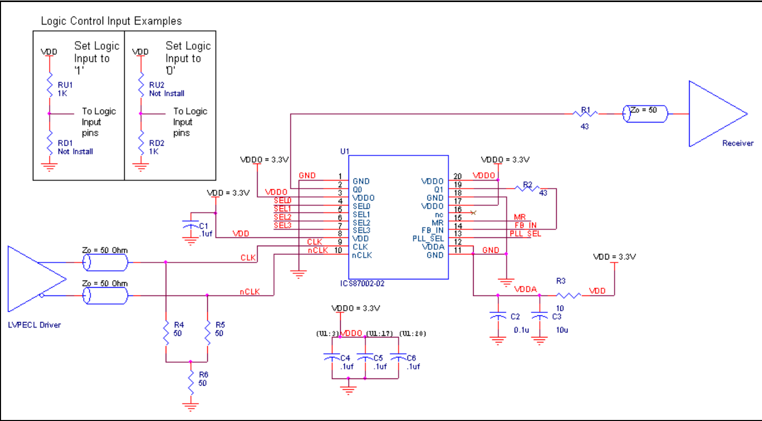
Figure 4. 87002-02 Schematic Example
