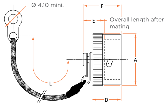
ATTACHED TO SQUARE FLANGE RECEPTACLE TYPE 00 C
