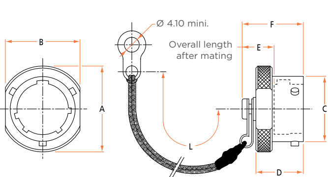
ATTACHED TO ACCESSORY (CABLE CLAMP) TYPE 06 C
