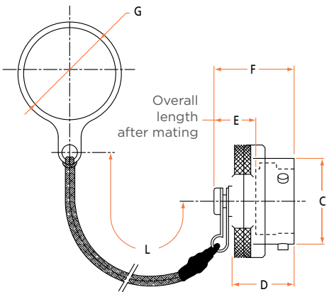
ATTACHED TO PLUG HOUSING TYPE 06-06 C
