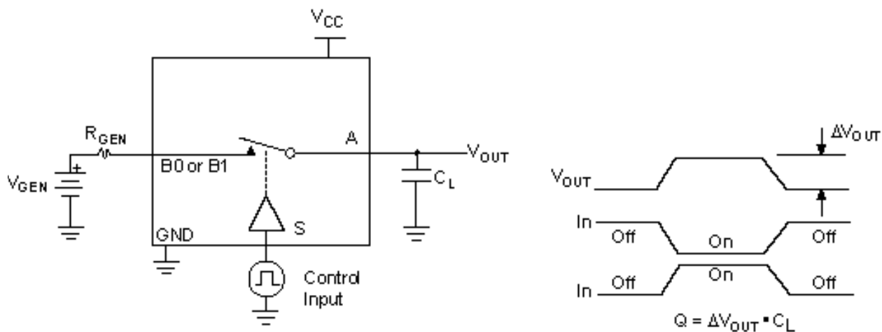
Figure 14. Charge Injection
