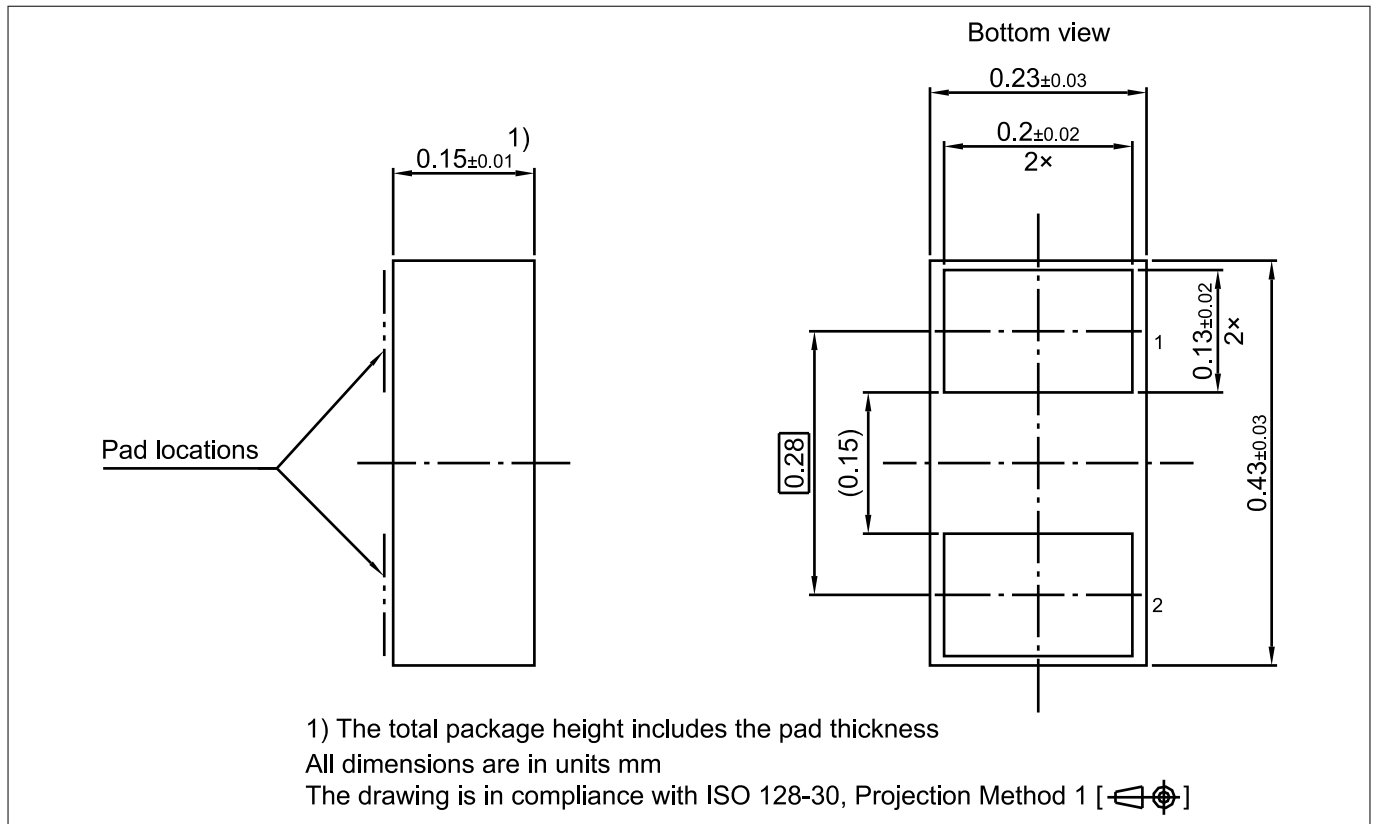
Figure 13 WLL-2-2 package
