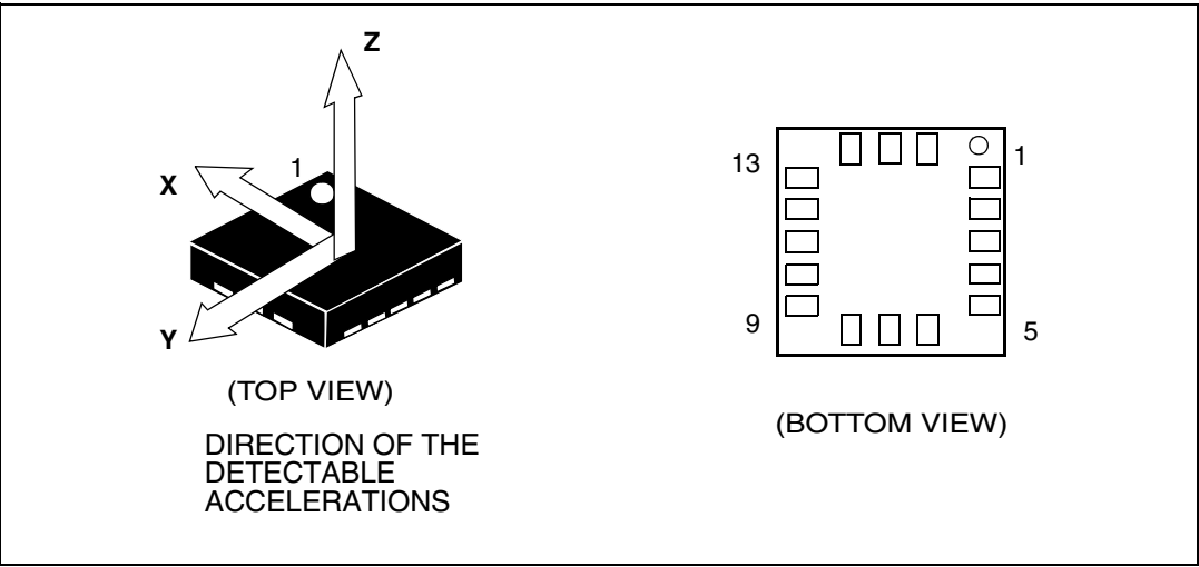
Figure 2. Pin connection
