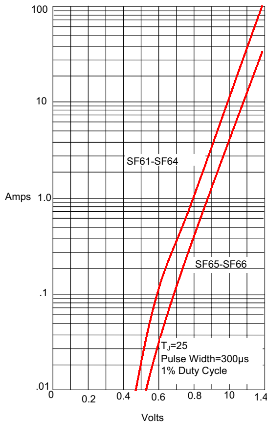
Figure 4 Typical Forward Characteristics
