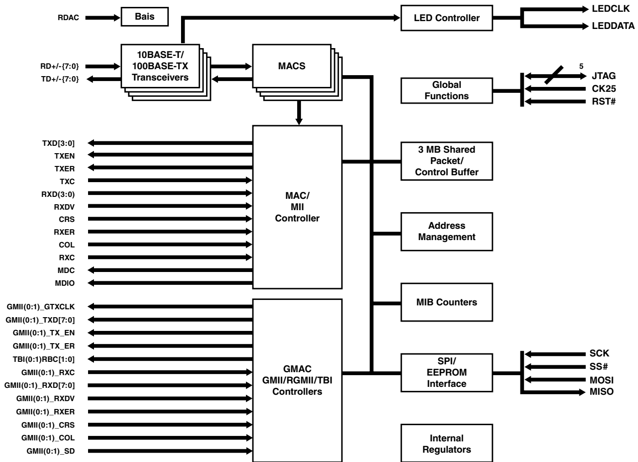
BCM53202M Block Diagram
