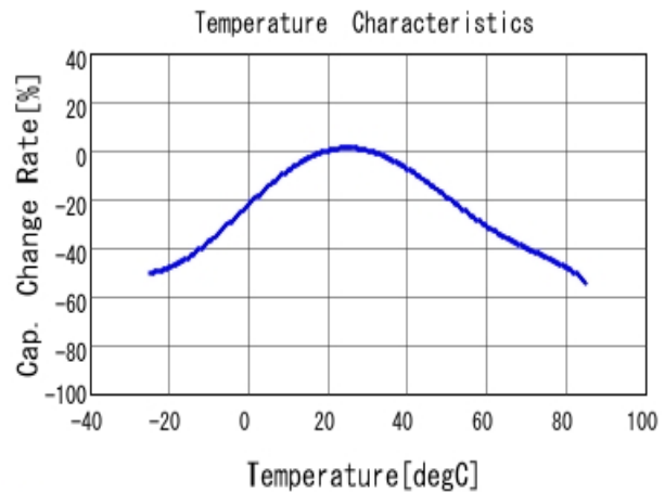
■ DE2E3SA152MA3BT02F C-Temp. capchange, DCOV, AC1Vrms
