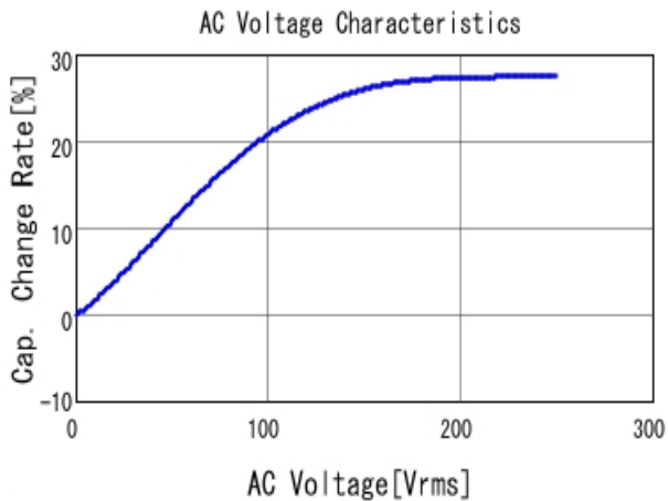
■ DE2E3SA152MA3BT02F C-AC Voltage capchange, DCOV, 20.0
