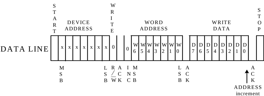
Figure 14. Write Operation
