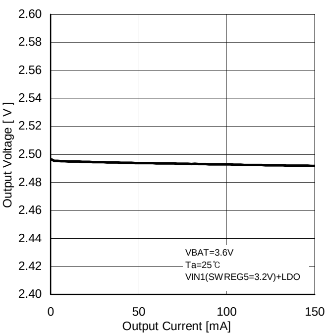
Figure 37. Output Voltage vs Output Current (LDO8 Load Regulation)
