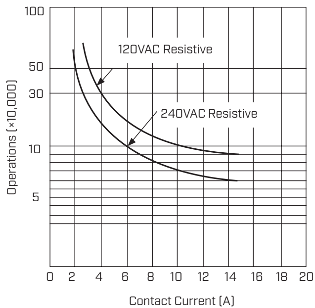
Life Curve
